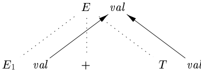
Figure 5.6: E.val is synthesized from E_1.val and T.val
